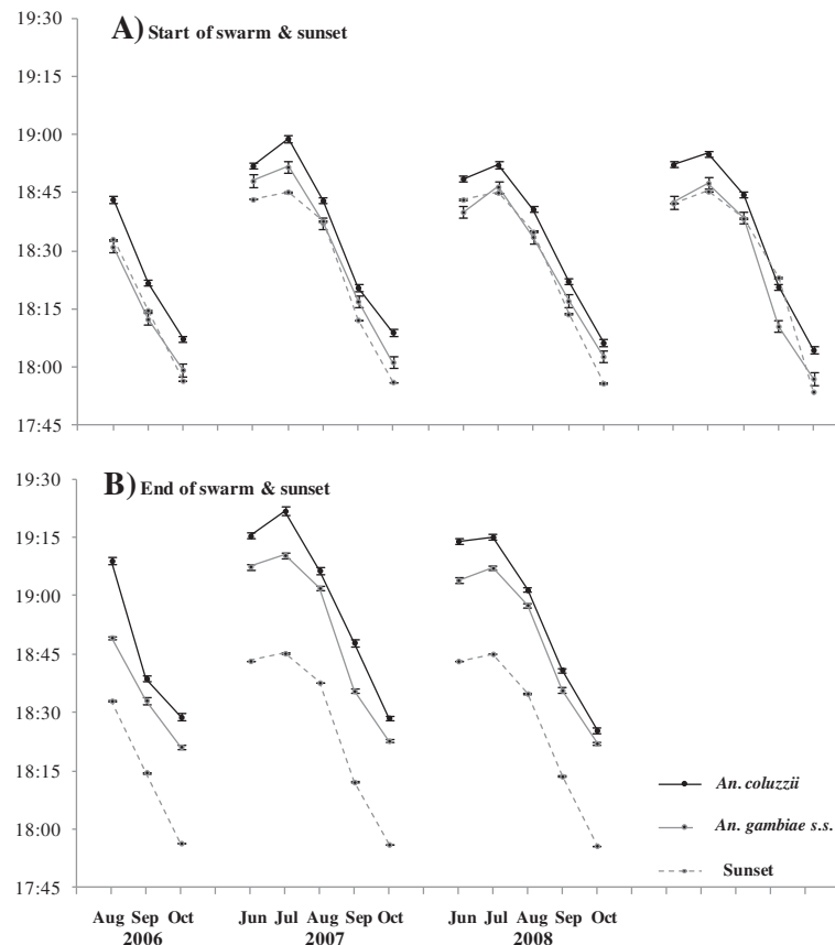
Figure 4 Relative timing of sunset and the start and end of swarming for Anopheles coluzzii and An. gambiae s.s. males across four rainy seasons. A) Start of swarming and sunset, B) End of swarming and sunset. Mean \pm s.e. times for An. gambiae s.s. normalised to sunset times in VK7 to take into account the effect of the difference in latitude and longitude between the two monitoring sites (VK7 and Soumouso) on the 'clock times' of sunset and the start and end of swarming (see Data analysis test). For each data point, n = 20 (for each species, the same five swarm sites monitored on four consecutive days each month). Note: the end of swarming was not recorded for 2009.
