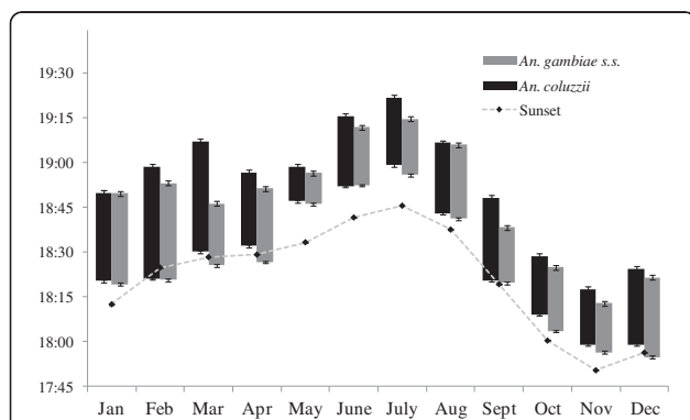
Figure 6 Duration of male swarms for Anopheles coluzzii in VK7 and An. gambiae s.s. in Soumoussou. Mean \pm s.e. times of the start and end of swarming (i.e., tops and bottoms of bars, respectively) in relation to the time of sunset each month in 2007 (n = 20 swarms/species/month). The 'duration' time of a swarm is the vertical length of each bar, based on the time scale of the y axis. Sunset and swarm times for Soumoussou normalised to VK7 'clock' times (see Figure 4 legend and Data analysis text). For sunset, s.e. = height of plotted points.
