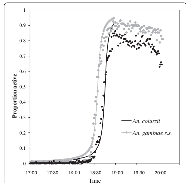
Figure 7 Comparison of the timing of onset of general dusk activity for male Anopheles coluzzii and An. gambiae s.s. in an actograph, September-October 2008. Cauchit curve fitted to data points for each species. Each data point indicates the proportion of males active in that minute, with n = six males of each species/night x 21 nights, i.e., 126 males of each species each minute, over 3 hours, i.e., 180 min).
