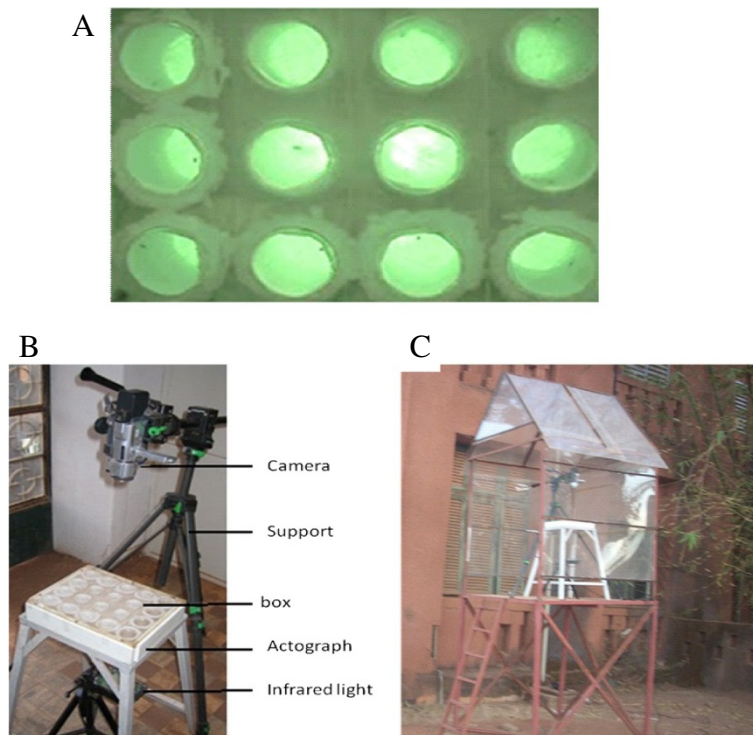
Figure 1 Actograph equipment to measure onset of spontaneous activity of individual male mosquitoes at dusk. A) arrangement of chambers that each hold a single mosquito, B) arrangement of video camera, actograph frame and infra-red lights, C) position of actograph apparatus within a protective framework, but exposed to ambient light, temperature and humidity.
