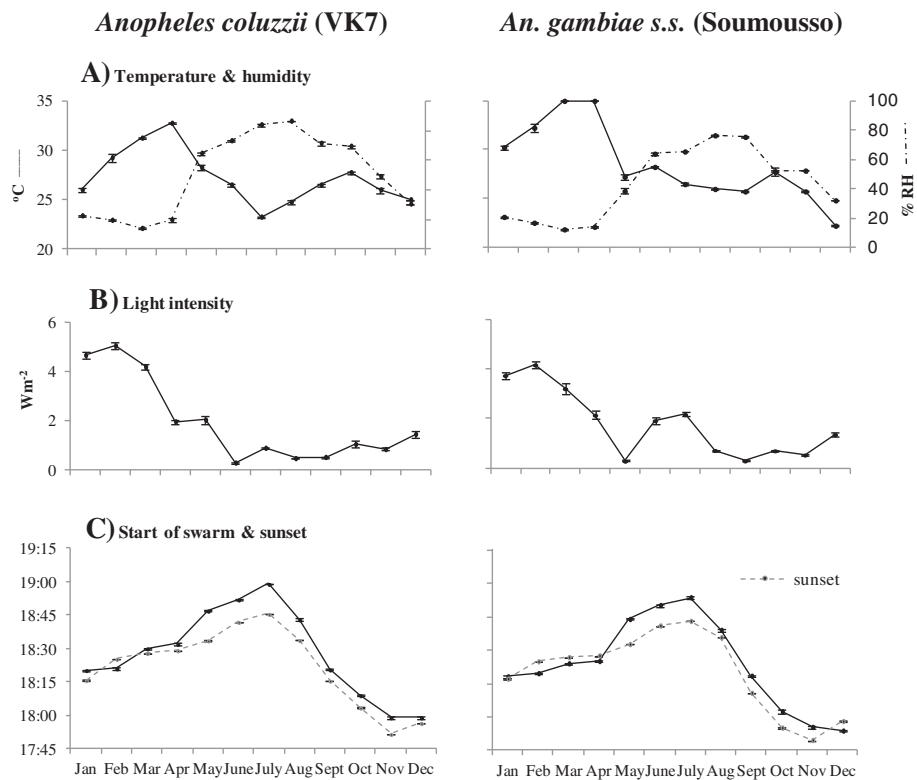
Figure 2 Relationships between the start of male swarming for Anopheles coluzzii (in VK7) and An. gambiae s.s. (in Soumouso) and environmental conditions. A) Mean \pm standard error (s.e.) temperature (solid line, left axis) and humidity (dashed line, right axis) when first male(s) observed swarming, B) light intensity at start of swarming and C) time at which first male(s) observed swarming (solid line) and time of sunset on swarm monitoring days. For each data point n = 20 (for each species, the same five swarm sites monitored on four consecutive days each month). Note: tick marks on the x-axis mark the boundaries between months.
